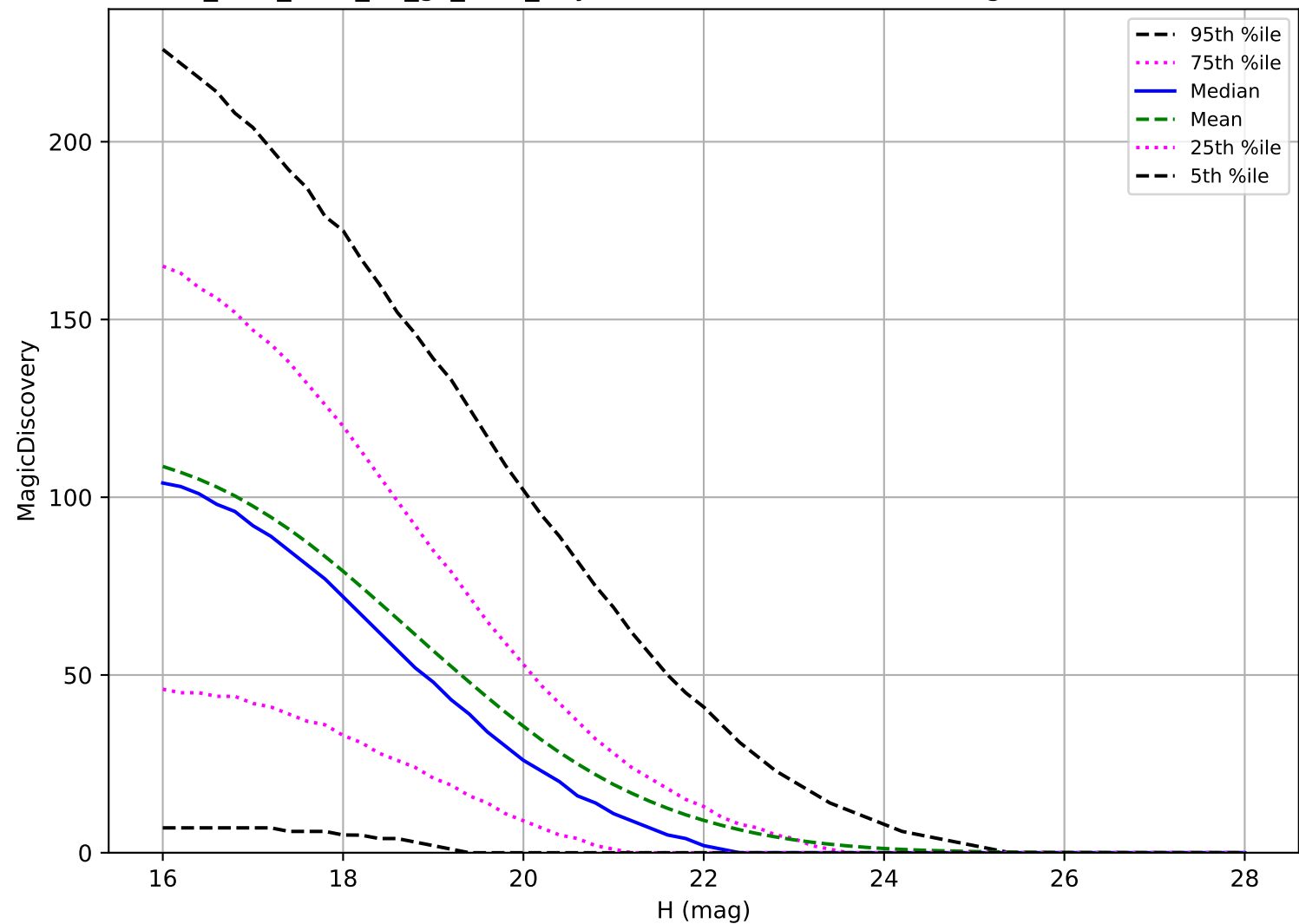
too_elab_r256_d2_gz_v3.4_10yrs: PHA 6 detections in 60 nights detection loss
