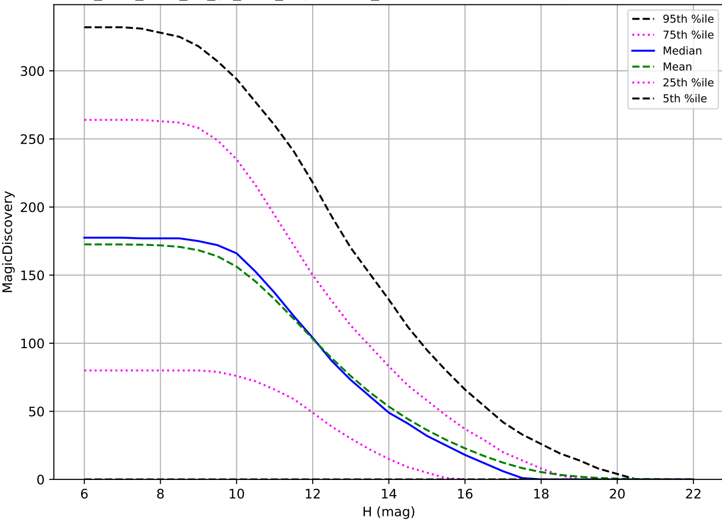
too_elab_r256_d2_gz_v3.4_10yrs: OCC_r5 6 detections in 60 nights detection loss
