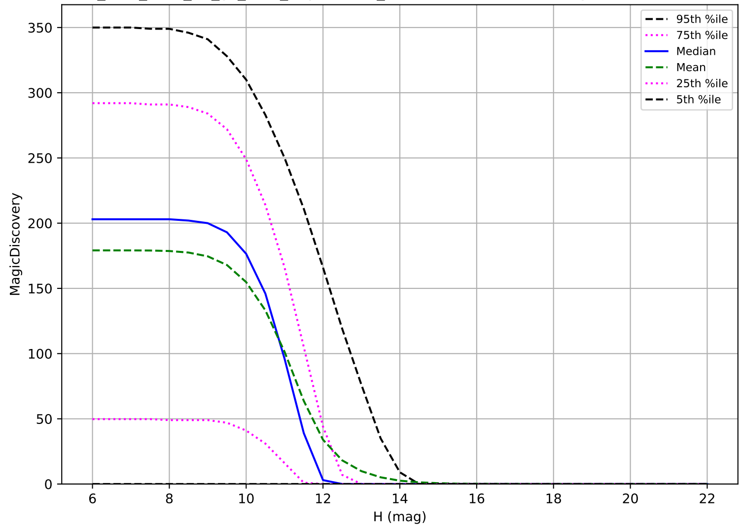
too_elab_r256_d2_gz_v3.4_10yrs: OCC_r20 6 detections in 60 nights detection loss
