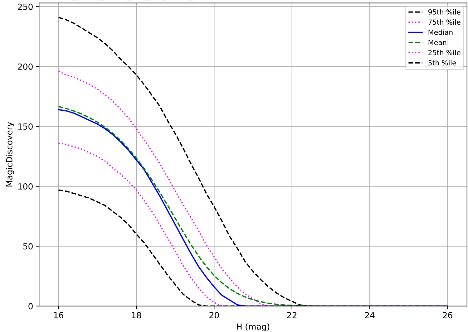
too_elab_r256_d2_gz_v3.4_10yrs: MBA 6 detections in 60 nights detection loss
