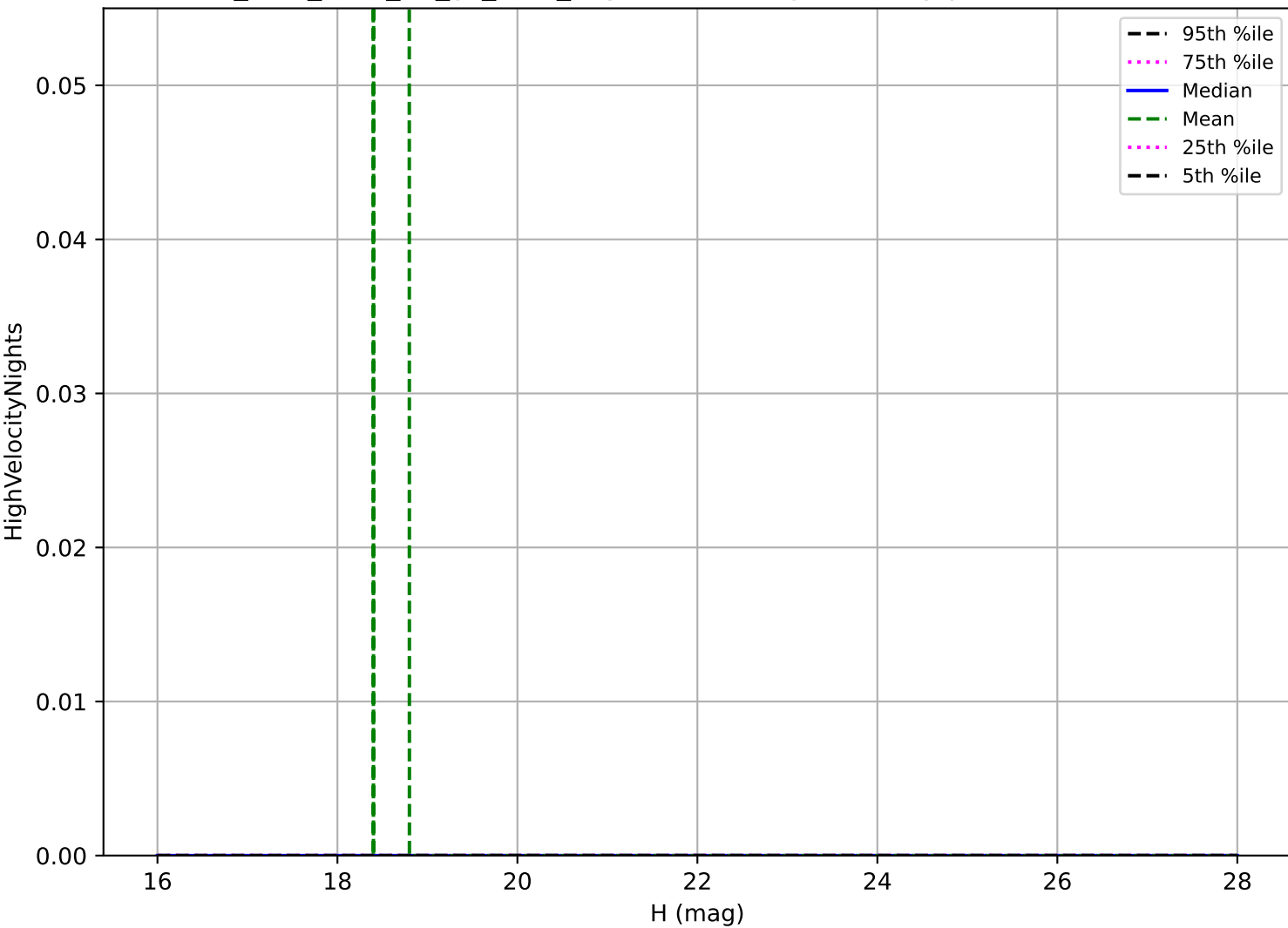
too_elab_r256_d2_gz_v3.4_10yrs: Vatira High velocity pair detection loss
