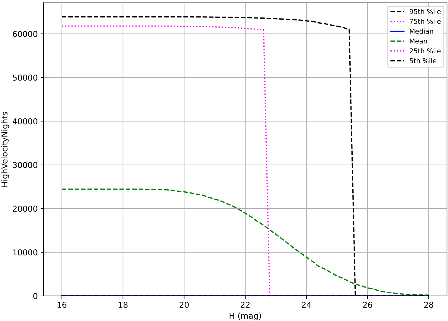
too_elab_r256_d2_gz_v3.4_10yrs: PHA High velocity pair detection loss
