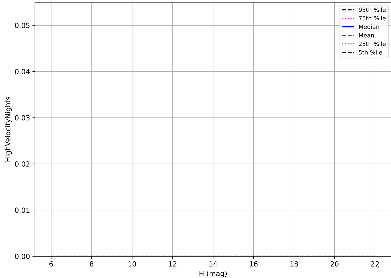
too_elab_r256_d2_gz_v3.4_10yrs: OCC_r5 High velocity pair detection loss
