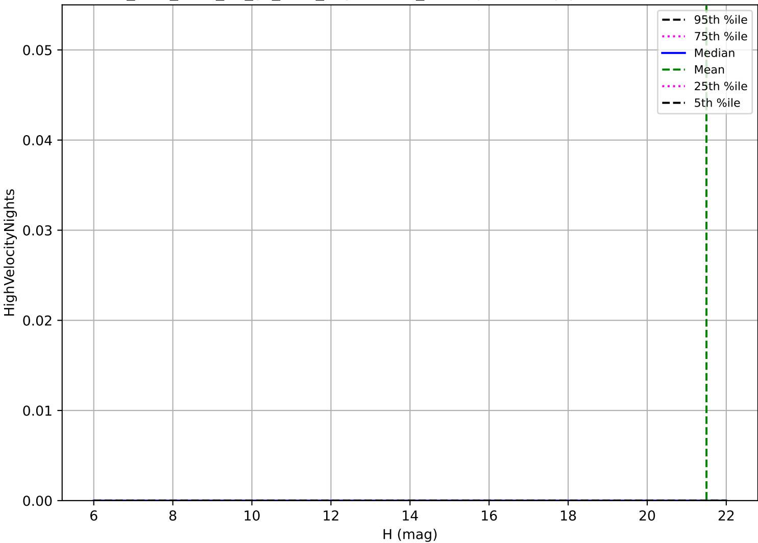
too_elab_r256_d2_gz_v3.4_10yrs: OCC_r20 High velocity pair detection loss
