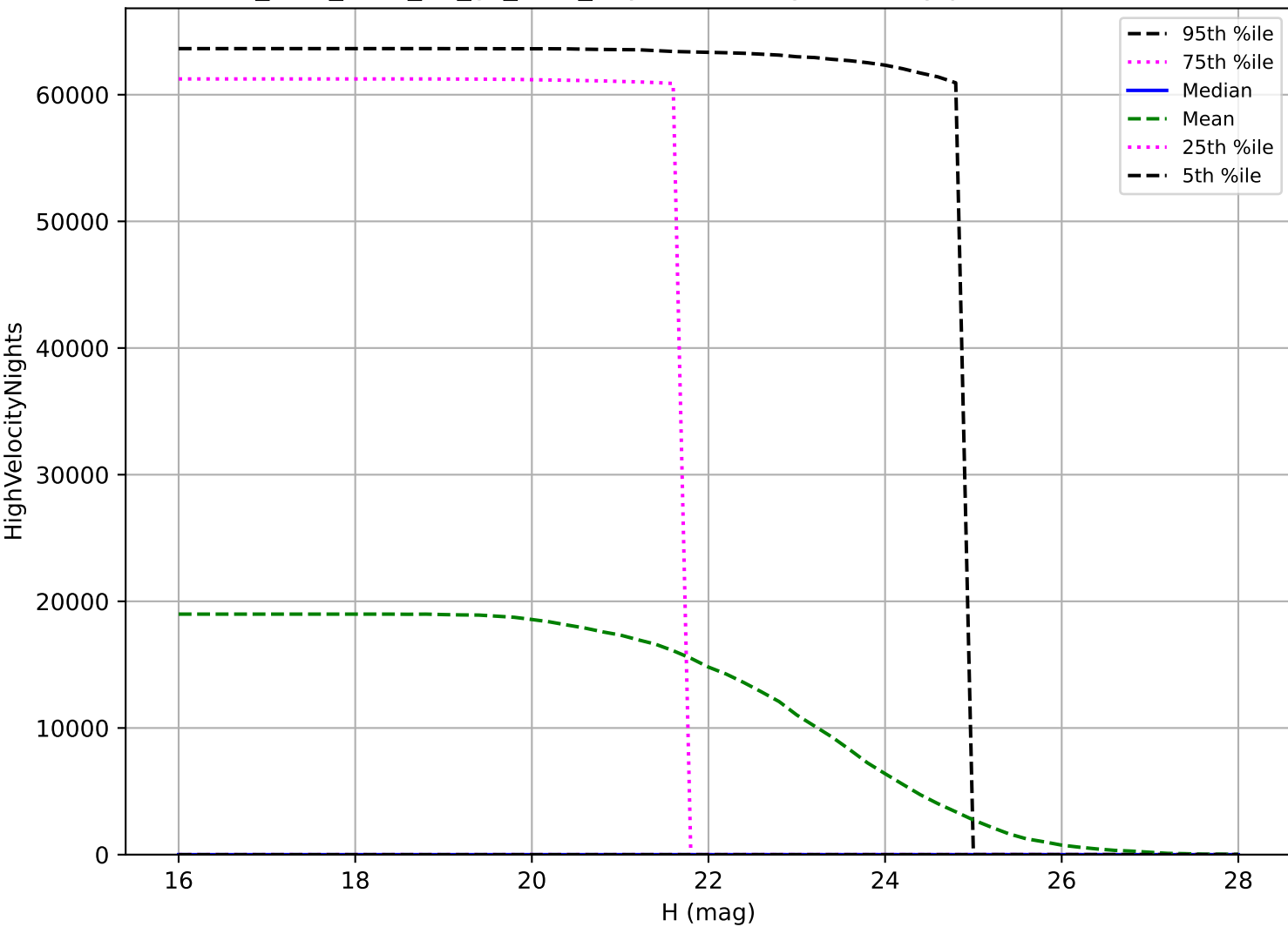
too_elab_r256_d2_gz_v3.4_10yrs: NEO High velocity pair detection loss
