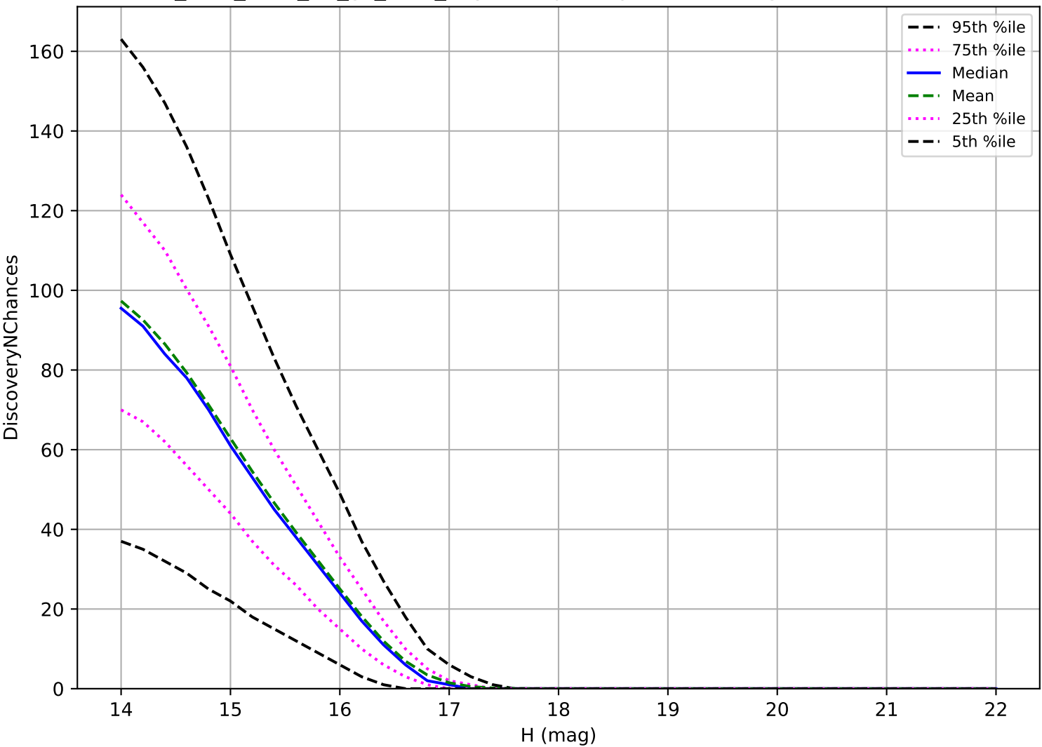
too_elab_r256_d2_gz_v3.4_10yrs: Trojan 3 pairs in 15 nights detection loss
