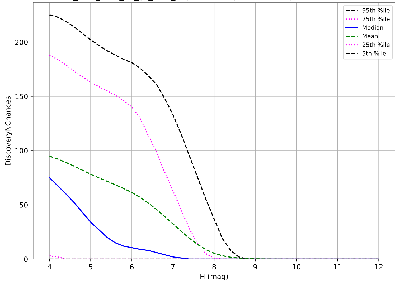
too_elab_r256_d2_gz_v3.4_10yrs: TNO 3 pairs in 15 nights detection loss
