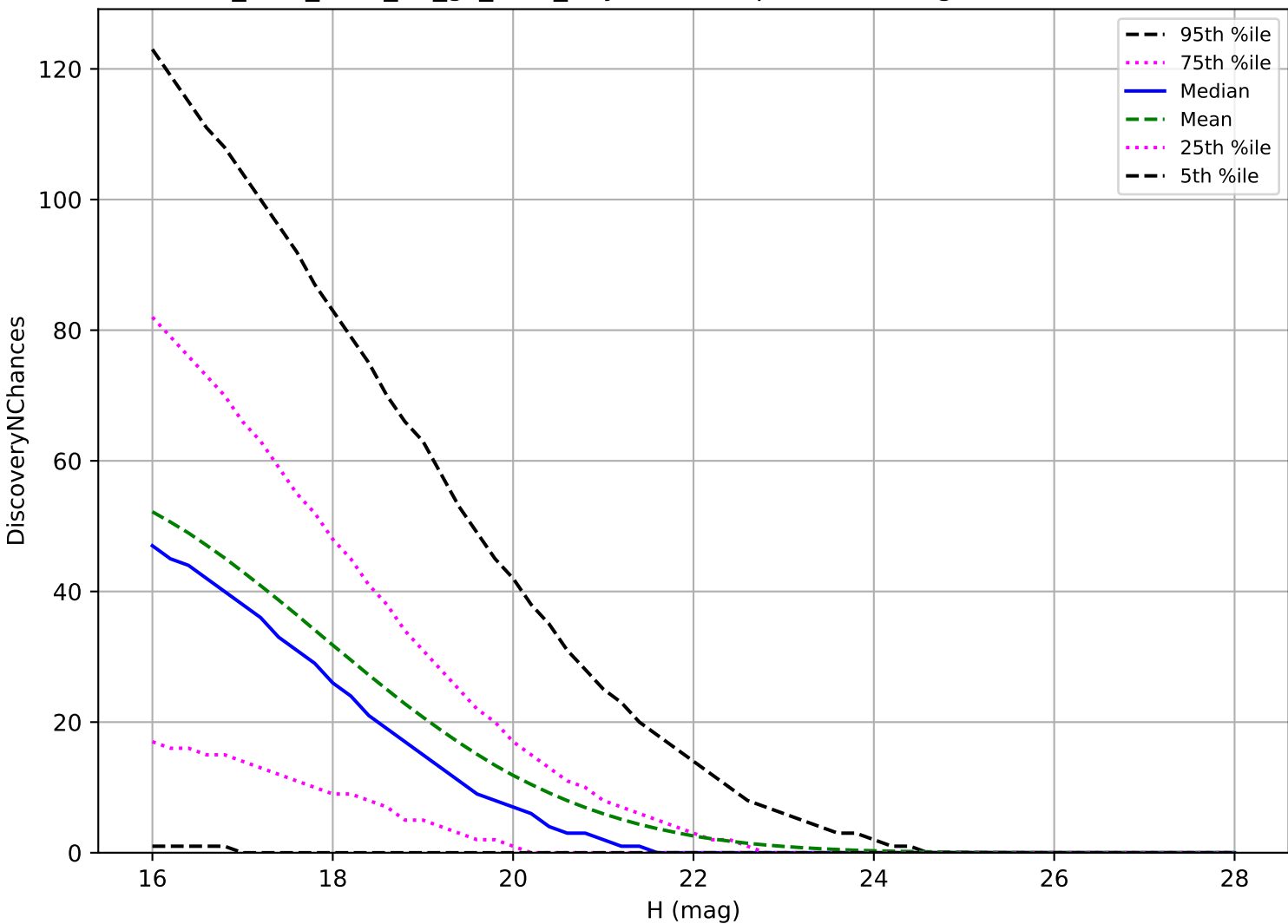
too_elab_r256_d2_gz_v3.4_10yrs: PHA 3 pairs in 15 nights detection loss
