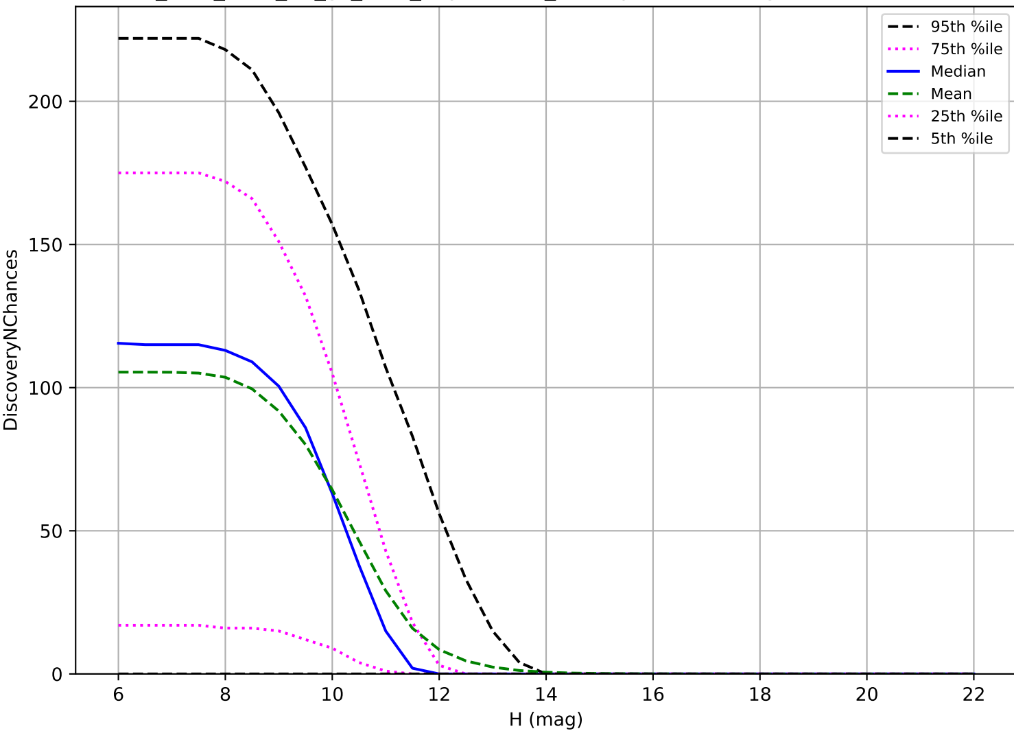
too_elab_r256_d2_gz_v3.4_10yrs: OCC_r20 3 pairs in 15 nights detection loss
