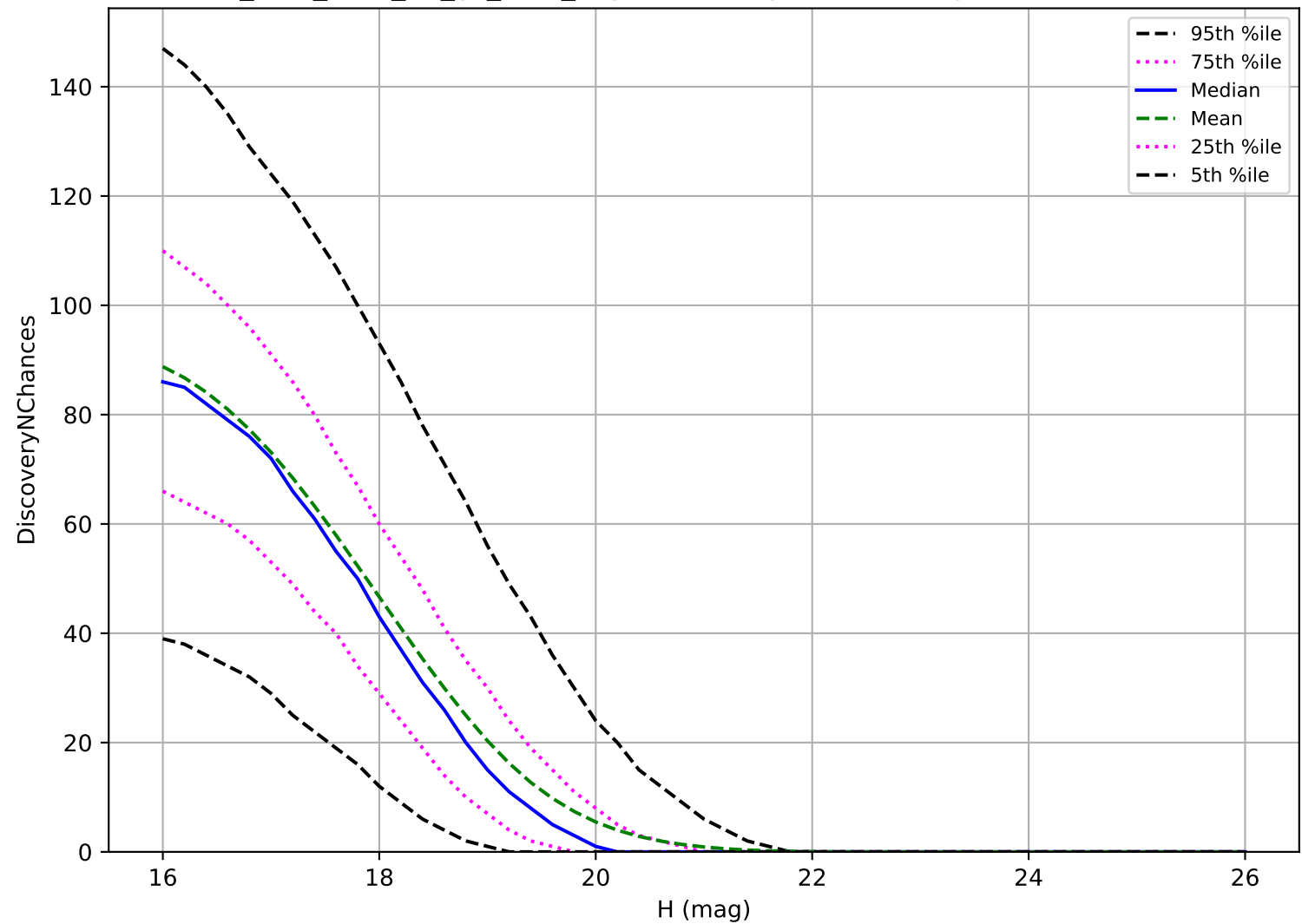
too_elab_r256_d2_gz_v3.4_10yrs: MBA 3 pairs in 15 nights detection loss
