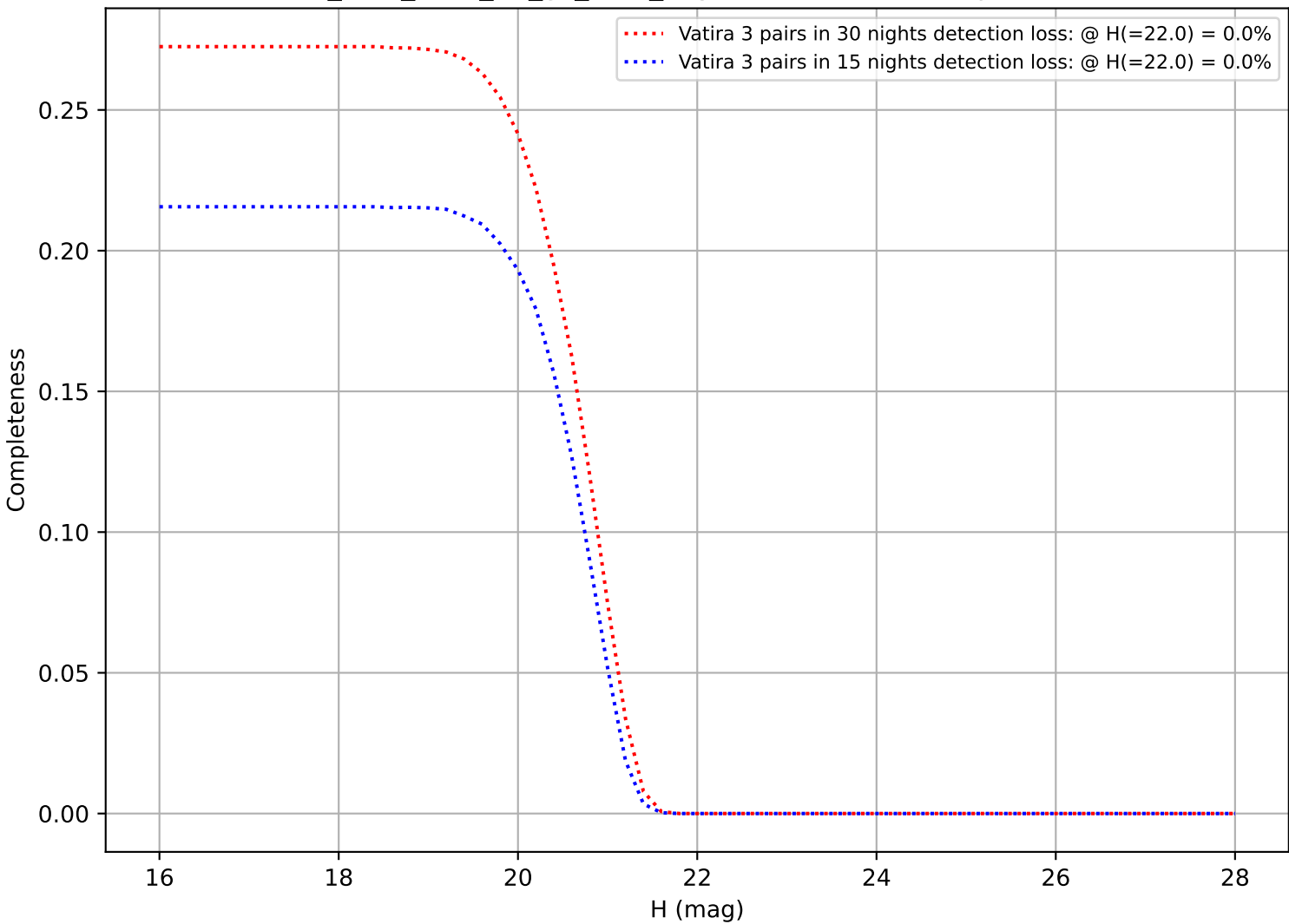
too_elab_r256_d2_gz_v3.4_10yrs: DifferentialCompleteness
