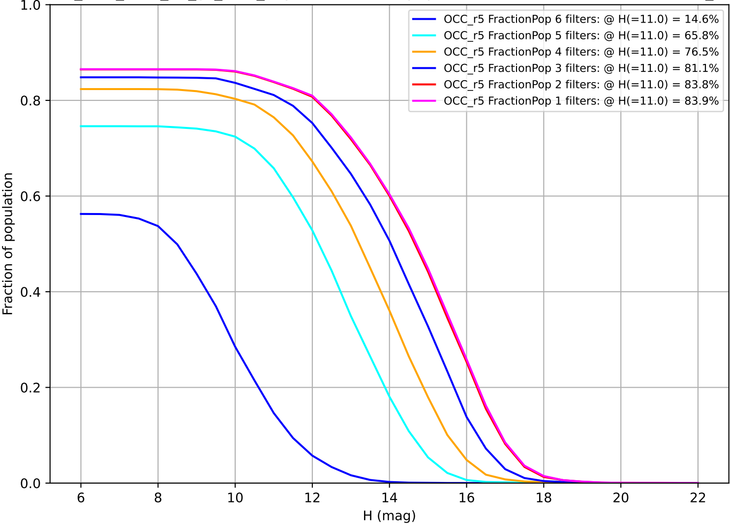
too_elab_r256_d2_gz_v3.4_10yrs: Fraction of population with colors in X filters OCC_r5
