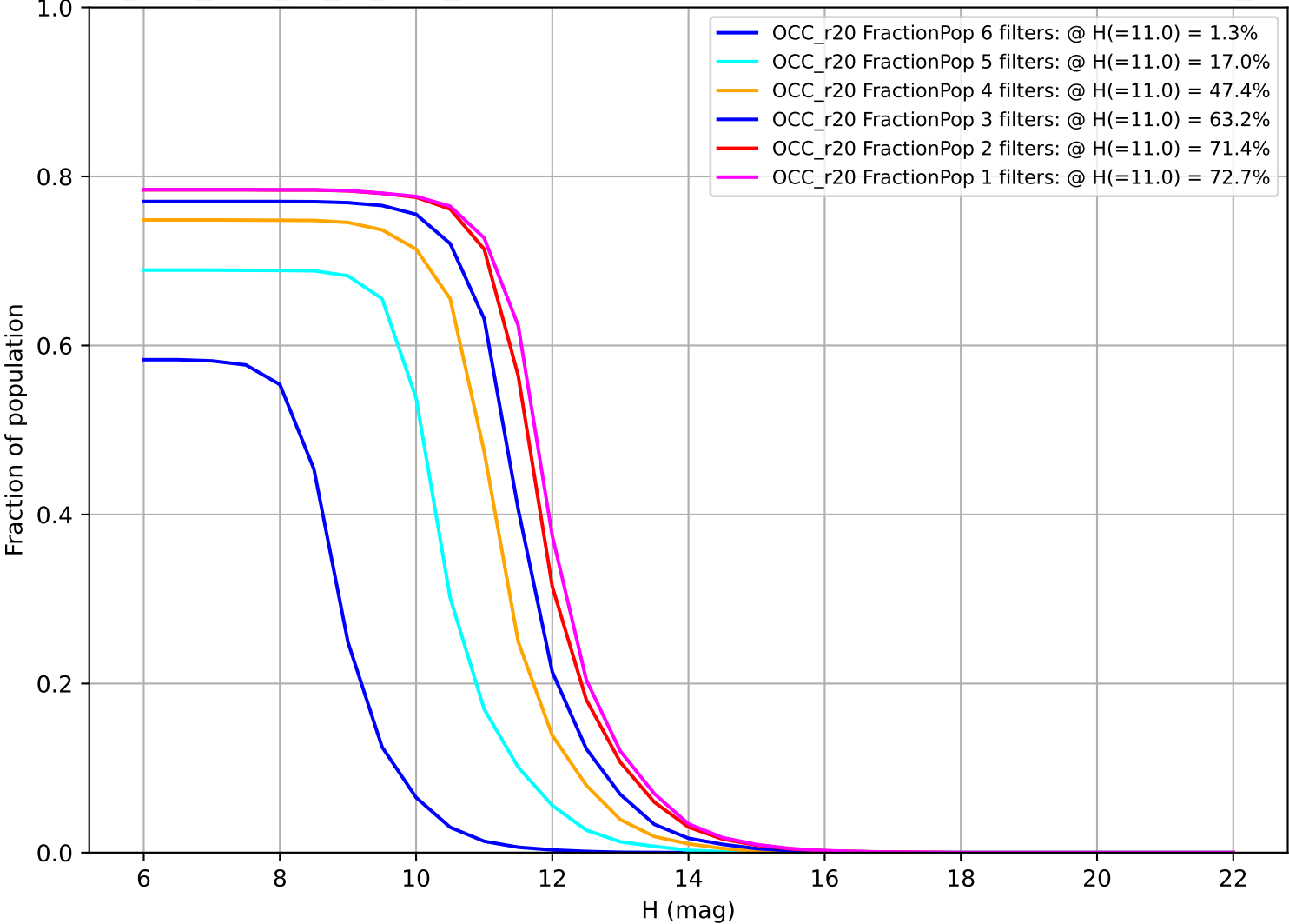
too_elab_r256_d2_gz_v3.4_10yrs: Fraction of population with colors in X filters OCC_r20
