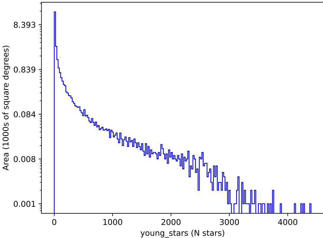
too_elab_r256_d2_gz_v3.4_10yrs : young_stars
