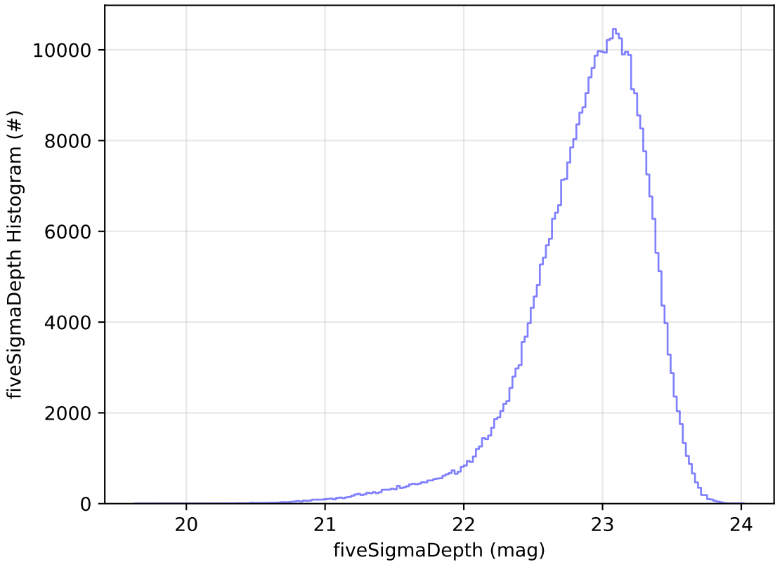
too_elab_r256_d2_gz_v3.4_10yrs z: fiveSigmaDepth Histogram
