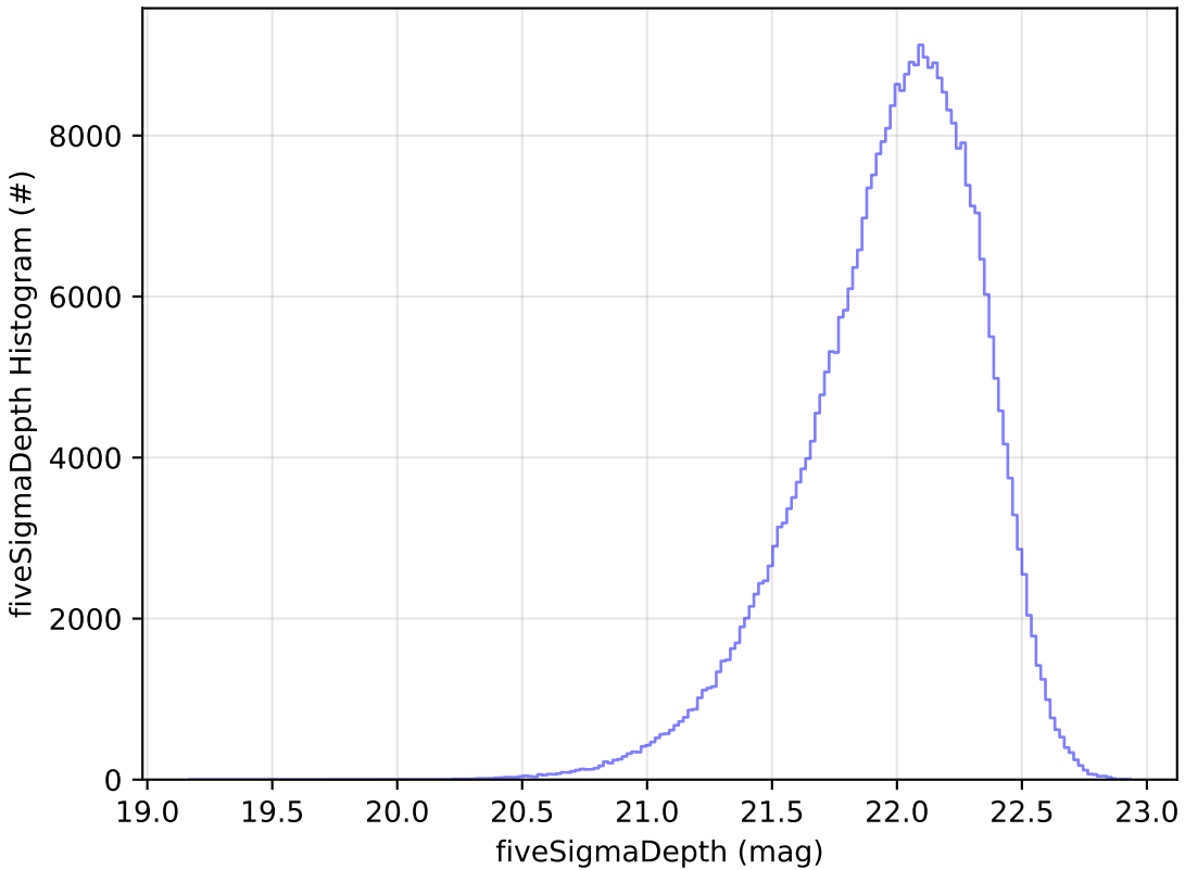
too_elab_r256_d2_gz_v3.4_10yrs y: fiveSigmaDepth Histogram
