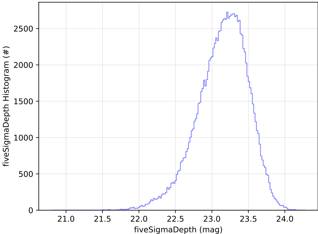
too_elab_r256_d2_gz_v3.4_10yrs u: fiveSigmaDepth Histogram
