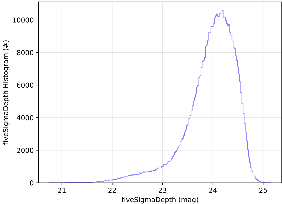
too_elab_r256_d2_gz_v3.4_10yrs r: fiveSigmaDepth Histogram
