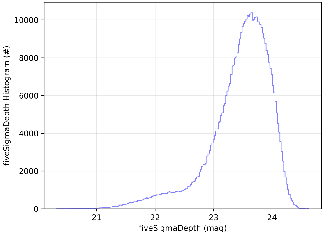
too_elab_r256_d2_gz_v3.4_10yrs i: fiveSigmaDepth Histogram
