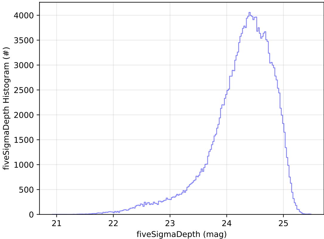
too_elab_r256_d2_gz_v3.4_10yrs g: fiveSigmaDepth Histogram
