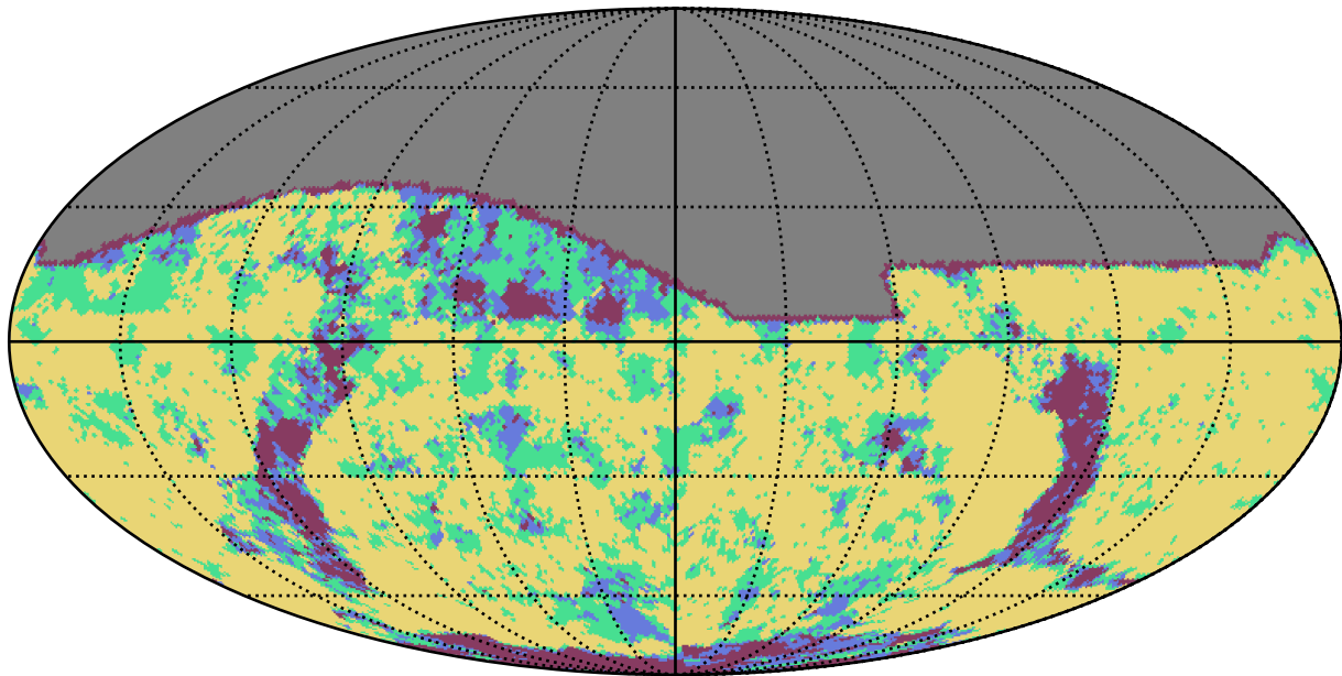
too_elab_r256_d2_gz_v3.4_10yrs g band: YearCoverage night
