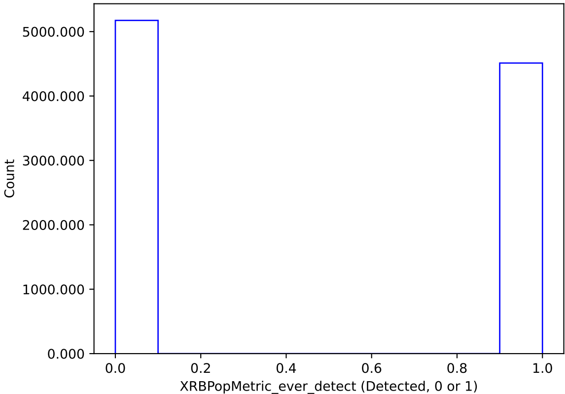
too_elab_r256_d2_gz_v3.4_10yrs : XRBPoMetric_ever_detect
