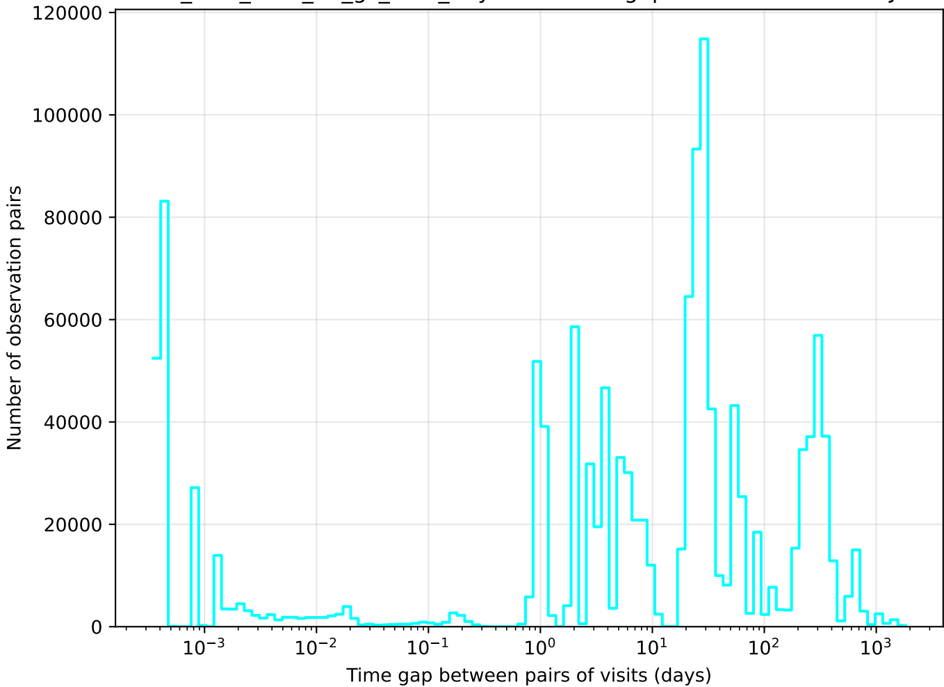
too_elab_r256_d2_gz_v3.4_10yrs u band: Tgaps observationStartMJD
