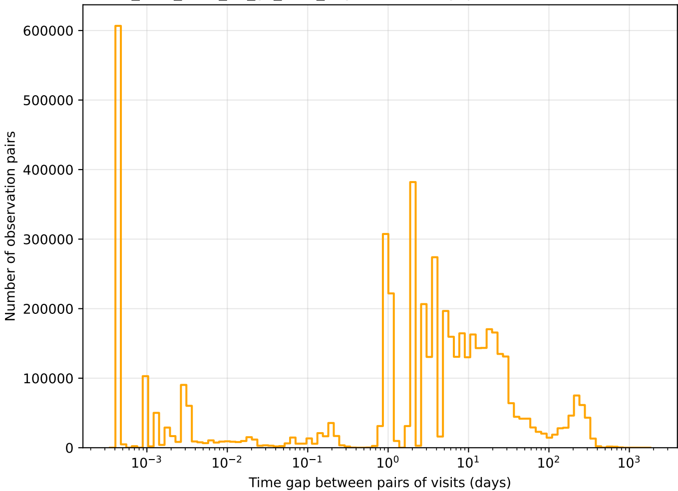
too_elab_r256_d2_gz_v3.4_10yrs r band: Tgaps observationStartMJD
