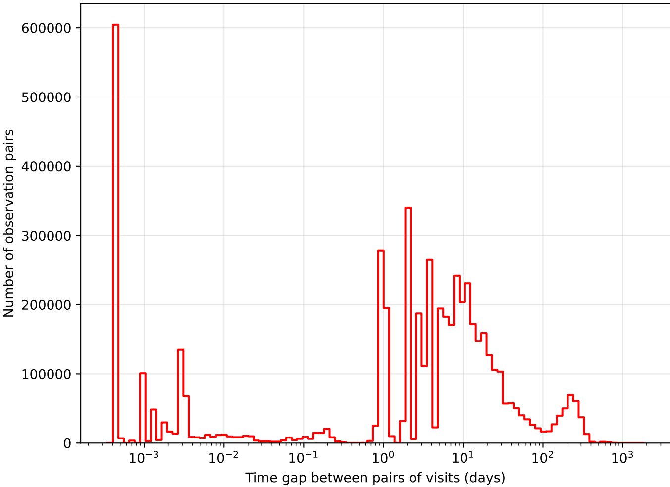
too_elab_r256_d2_gz_v3.4_10yrs i band: Tgaps observationStartMJD
