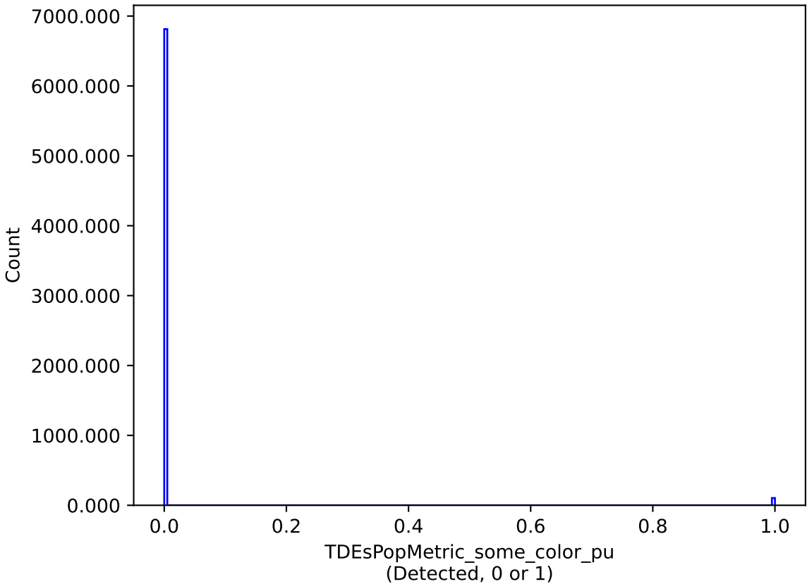
too_elab_r256_d2_gz_v3.4_10yrs : TDEsPopMetric_some_color_pu
