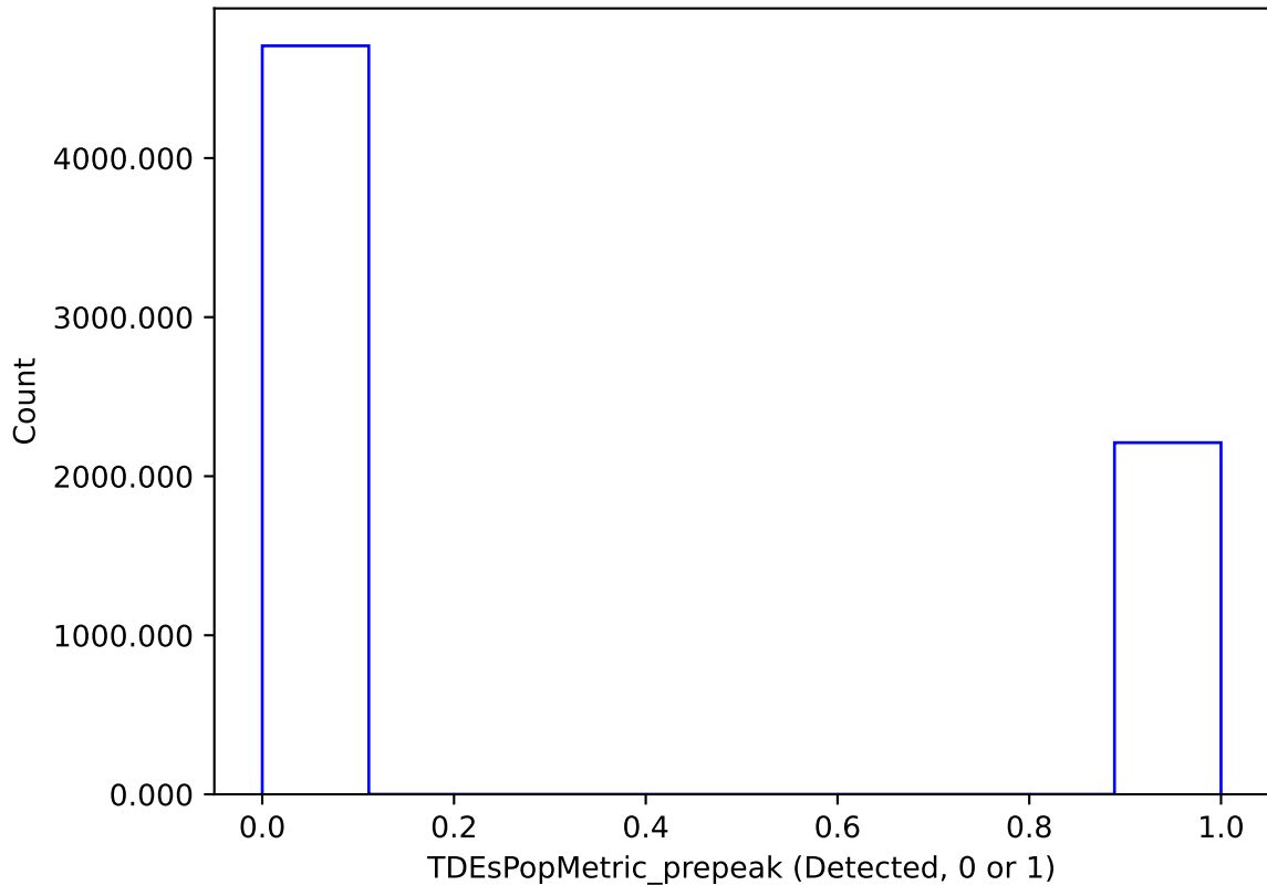
too_elab_r256_d2_gz_v3.4_10yrs : TDEsPopMetric_prepeak
