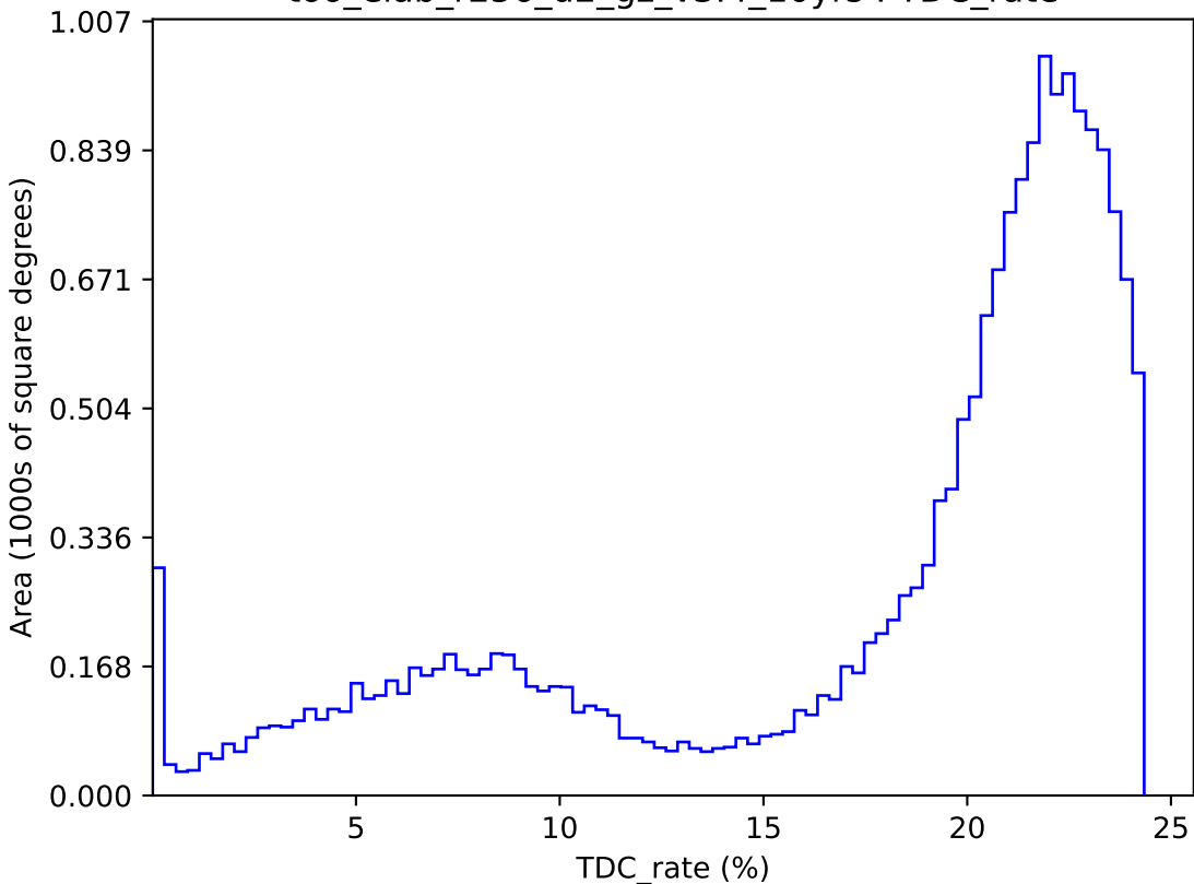
too_elab_r256_d2_gz_v3.4_10yrs : TDC_rate
