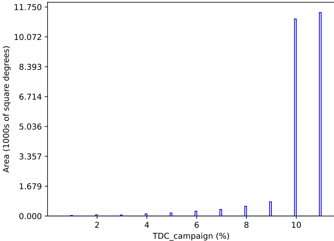
too_elab_r256_d2_gz_v3.4_10yrs : TDC_campaign
