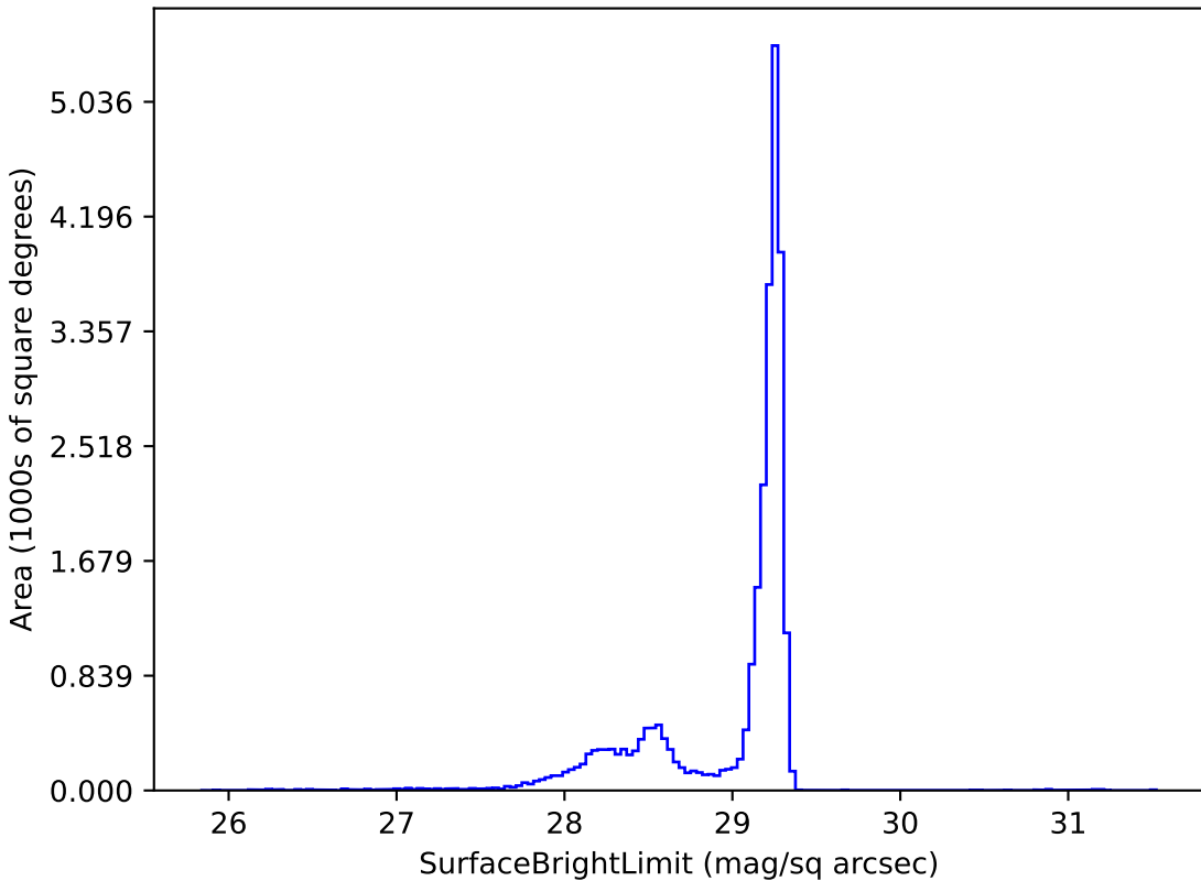
too_elab_r256_d2_gz_v3.4_10yrs z: SurfaceBrightLimit
