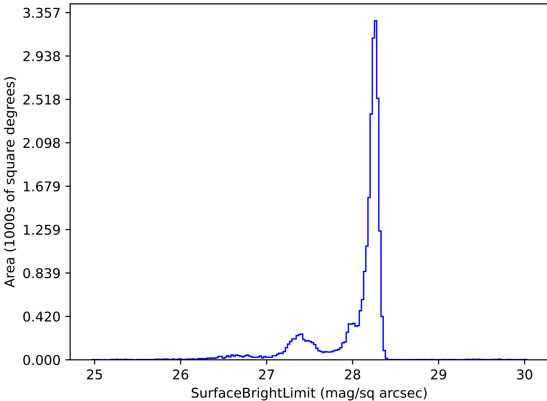
too_elab_r256_d2_gz_v3.4_10yrs y: SurfaceBrightLimit
