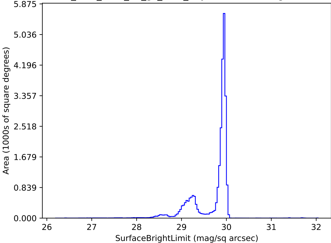
too_elab_r256_d2_gz_v3.4_10yrs i: SurfaceBrightLimit
