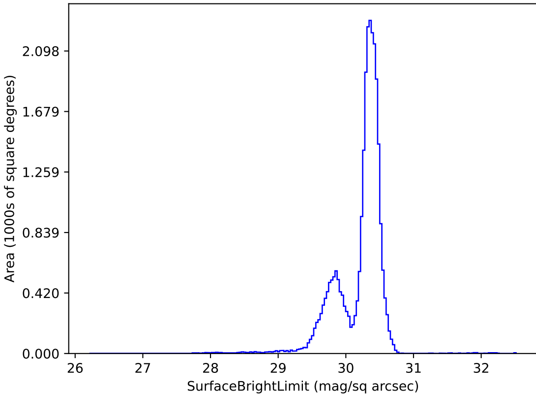
too_elab_r256_d2_gz_v3.4_10yrs g: SurfaceBrightLimit
