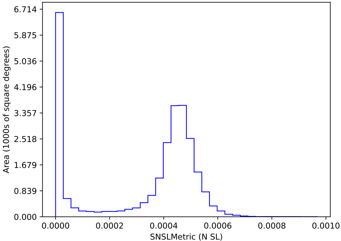
too_elab_r256_d2_gz_v3.4_10yrs : SNSLMetric
