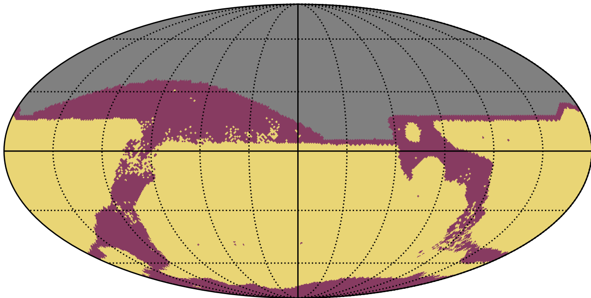
too_elab_r256_d2_gz_v3.4_10yrs : RapidRevisits
