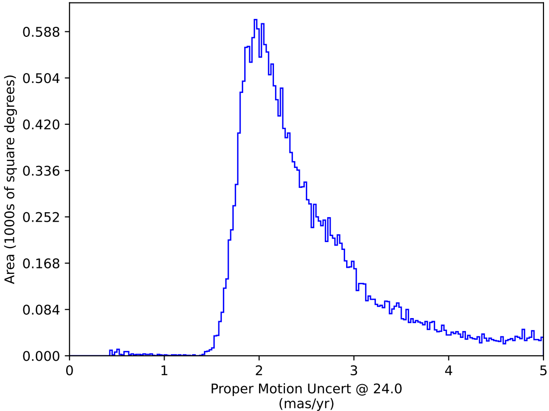
too_elab_r256_d2_gz_v3.4_10yrs : Proper Motion Uncert @ 24.0
