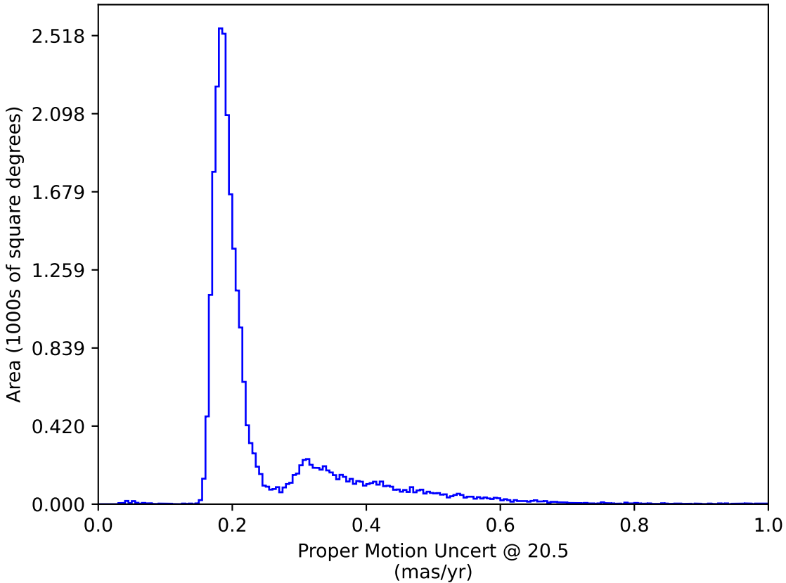
too_elab_r256_d2_gz_v3.4_10yrs : Proper Motion Uncert @ 20.5
