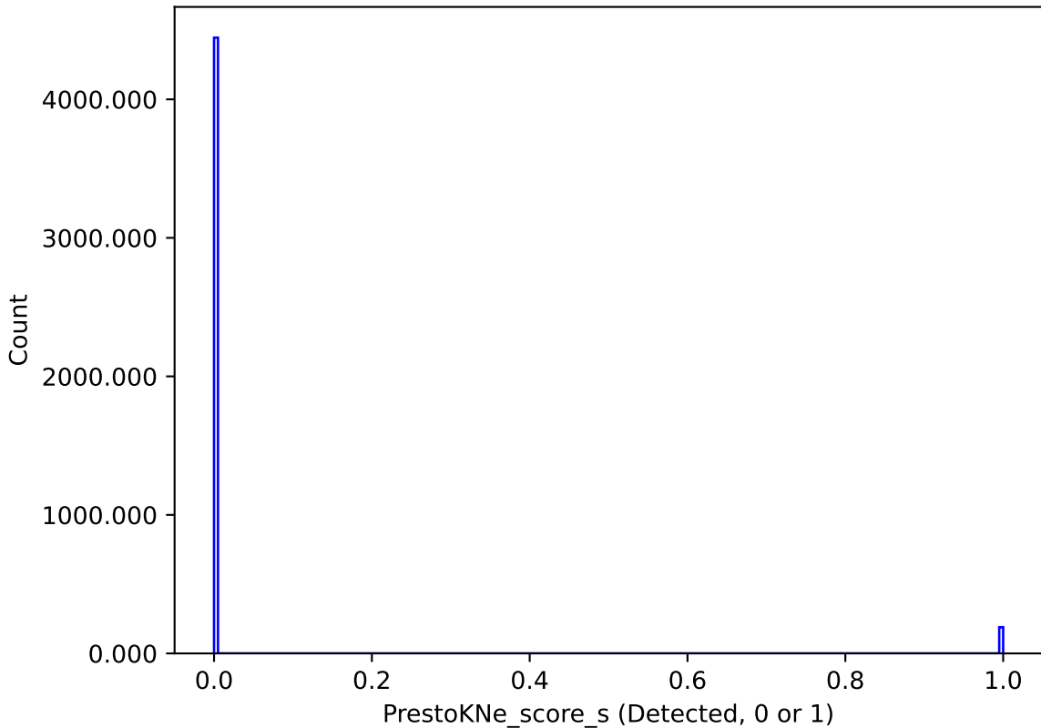
too_elab_r256_d2_gz_v3.4_10yrs : PrestoKNe_score_s
