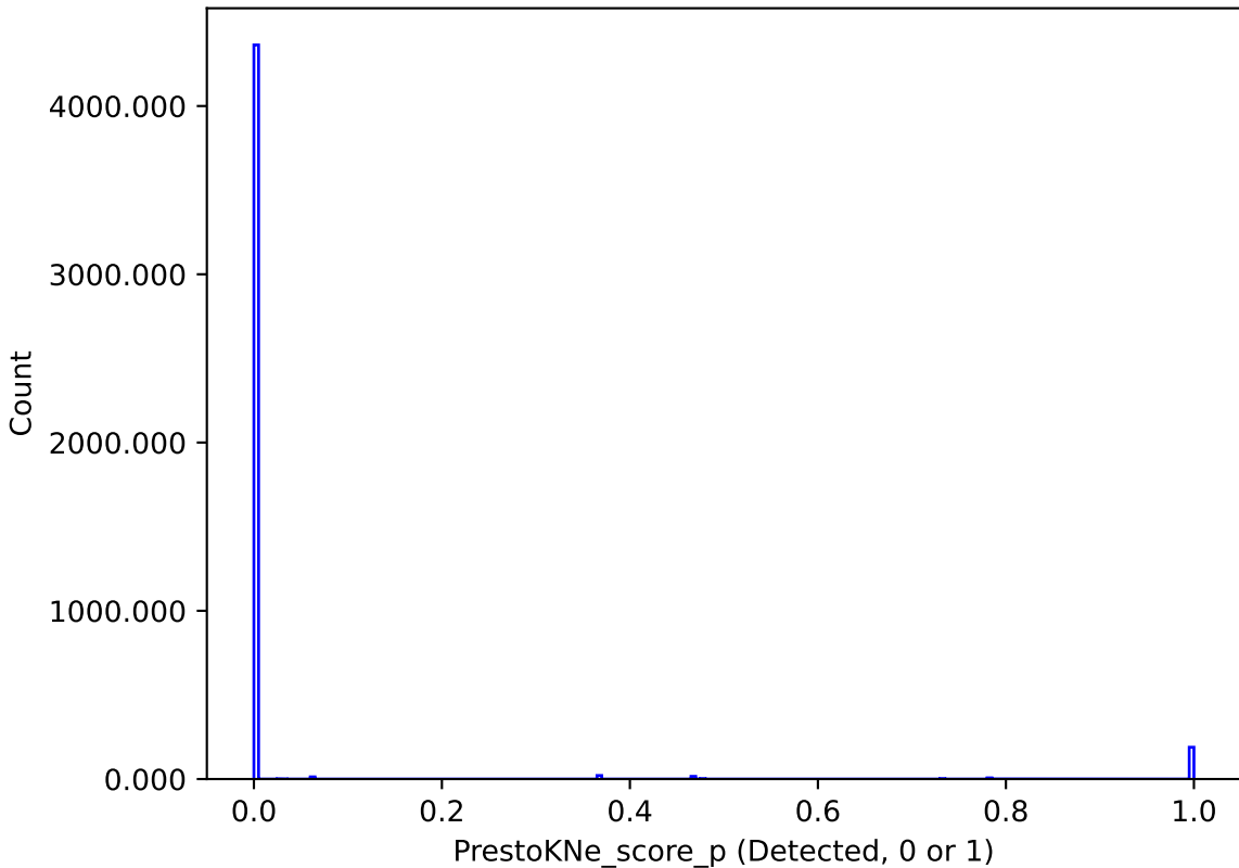
too_elab_r256_d2_gz_v3.4_10yrs : PrestoKNe_score_p
