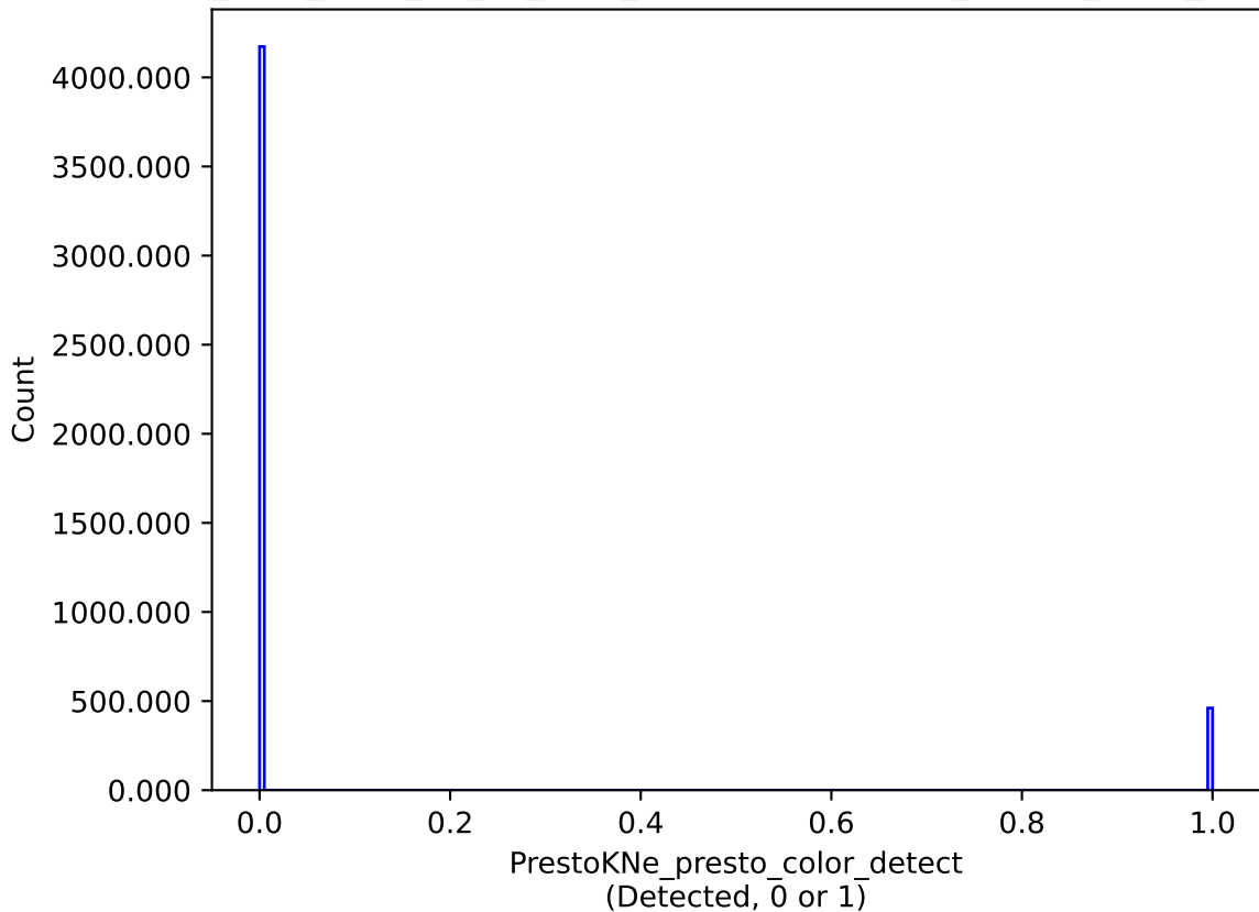
too_elab_r256_d2_gz_v3.4_10yrs : PrestoKNe_presto_color_detect
