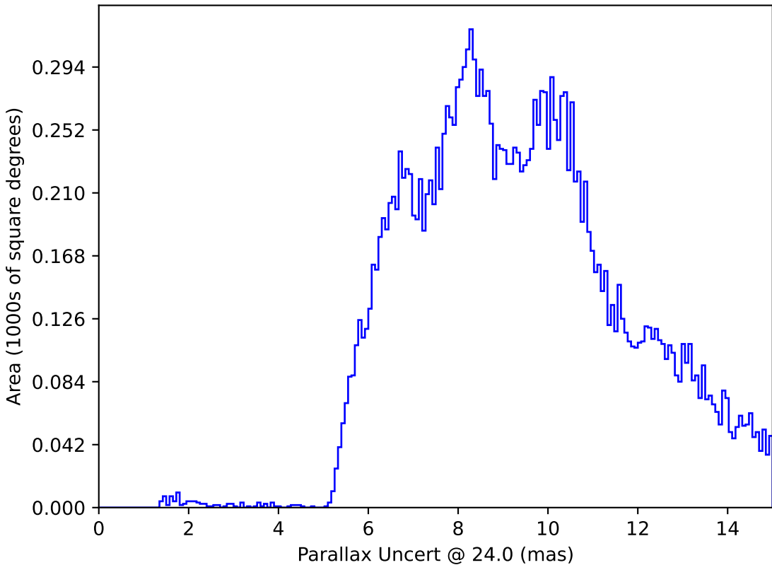
too_elab_r256_d2_gz_v3.4_10yrs : Parallax Uncert @ 24.0
