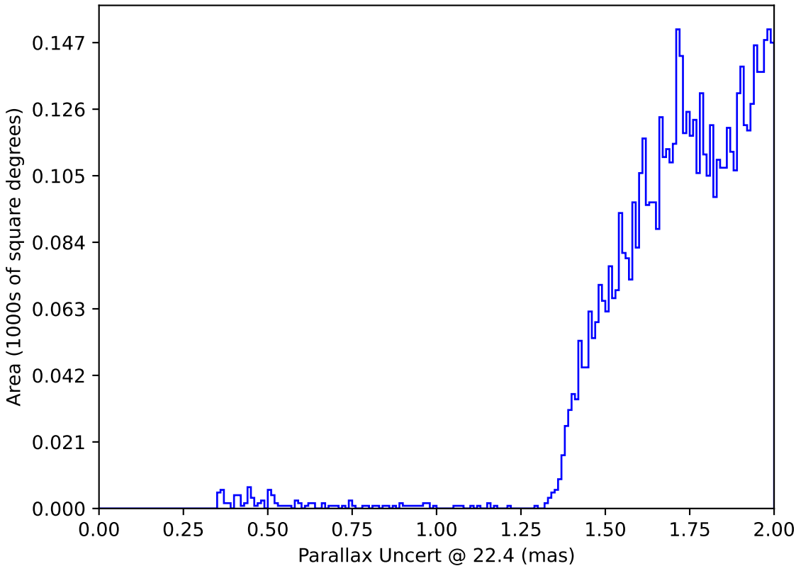
too_elab_r256_d2_gz_v3.4_10yrs : Parallax Uncert @ 22.4
