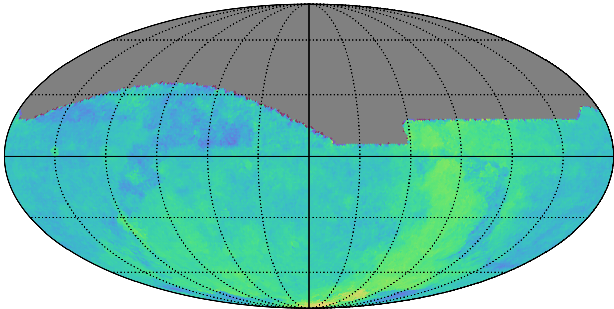
too_elab_r256_d2_gz_v3.4_10yrs : Parallax Coverage @ 24.0
