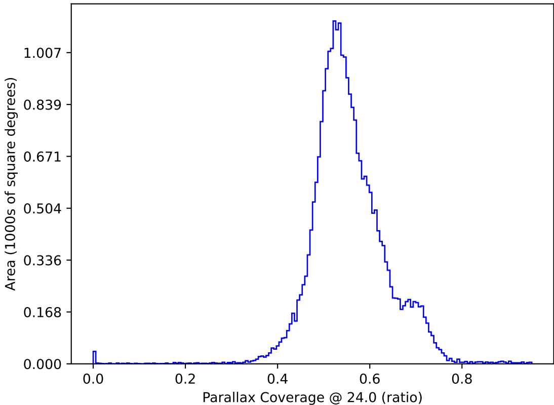
too_elab_r256_d2_gz_v3.4_10yrs : Parallax Coverage @ 24.0
