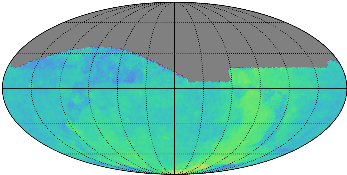
too_elab_r256_d2_gz_v3.4_10yrs : Parallax Coverage @ 22.4
