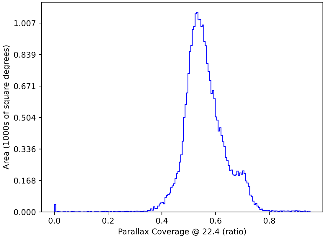
too_elab_r256_d2_gz_v3.4_10yrs : Parallax Coverage @ 22.4
